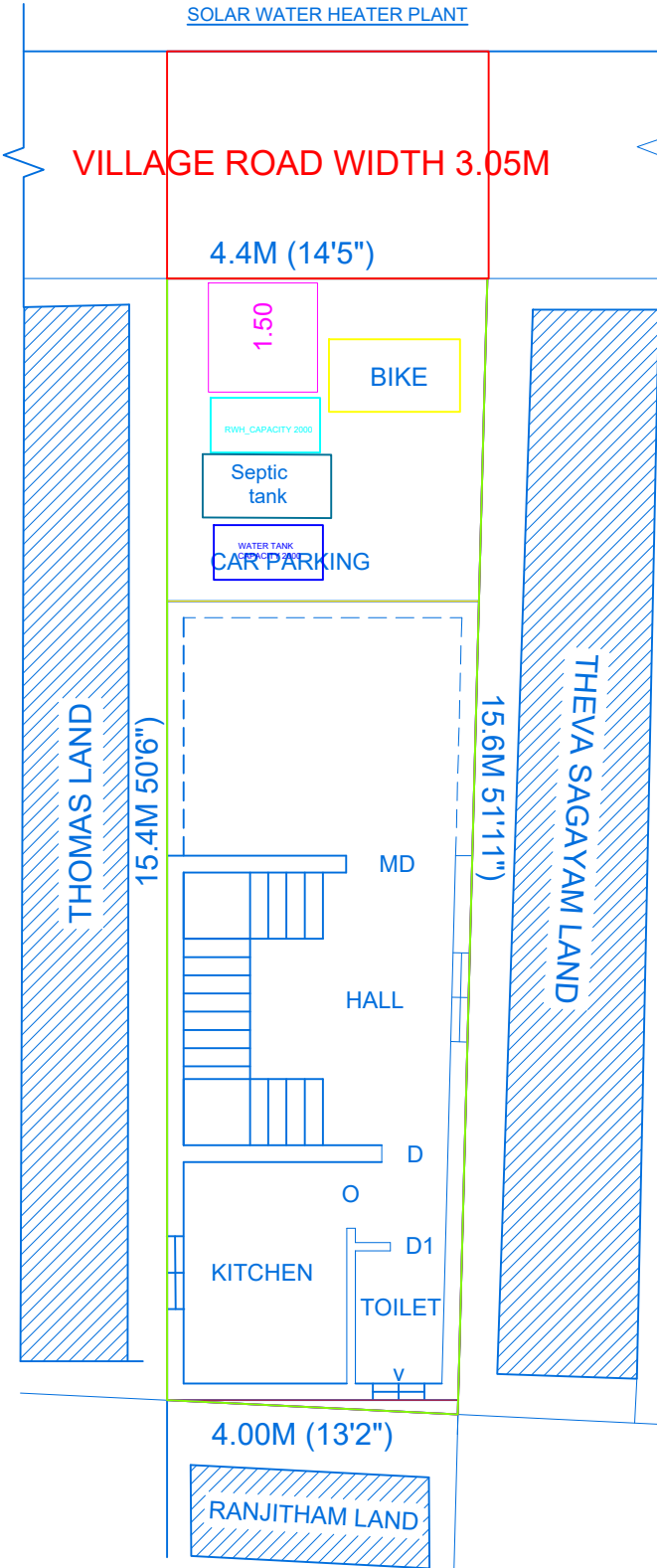
SITE PLAN
