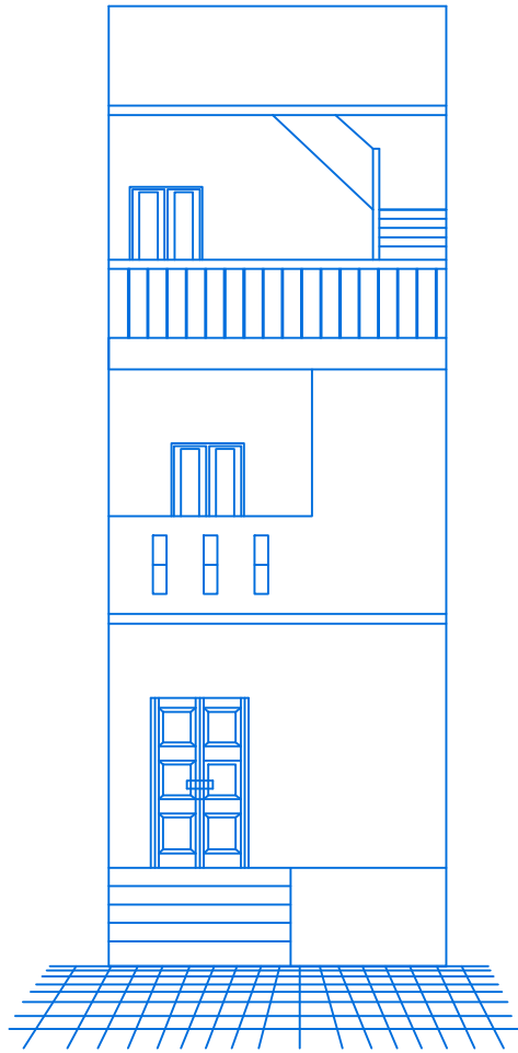
FRONT ELEVATION
