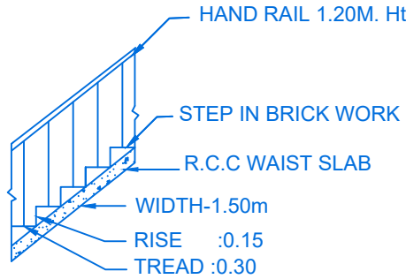
STAIR DETAIL
