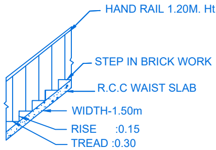
STAIR DETAIL
