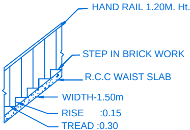
STAIR DETAIL
