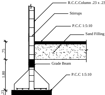
COLUMN DETAIL
