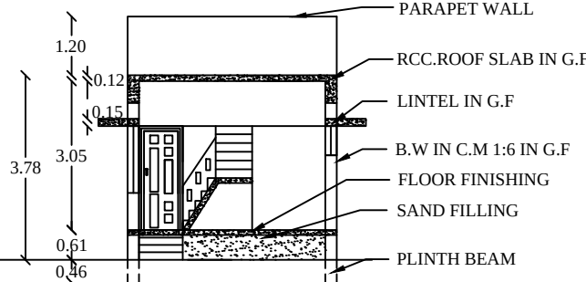
CROSS SECTION A-B
