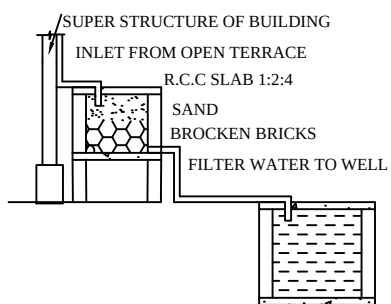
RAINWATER HARVESTING
