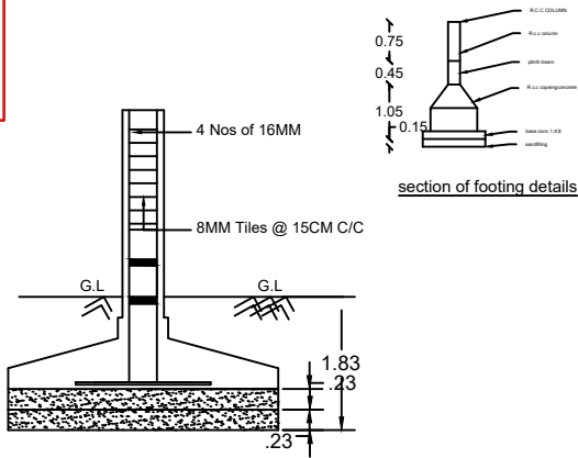
RCC COLUMN DETAILS
