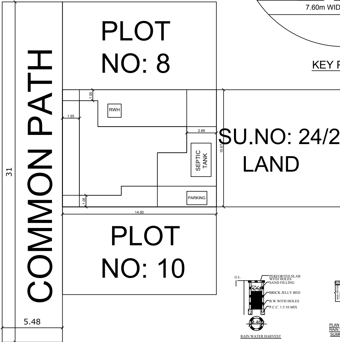
SITE PLAN
