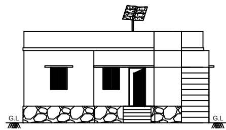
FRON ELEVATION
