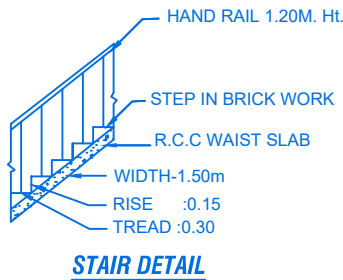
STAIR DETAIL
