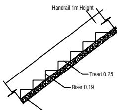
STAIR DETAILS
