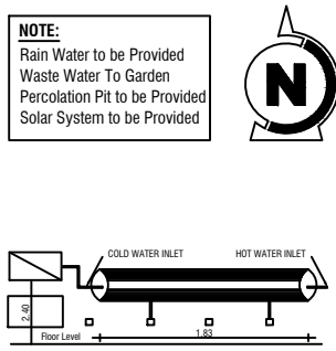
DETAILS OF SOLAR HOT WATER SYSTEM
