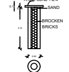
PERCOLATION PIT
