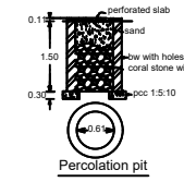
Percolation pit
