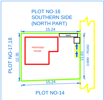
LOCATION PLAN Scale 1:400
