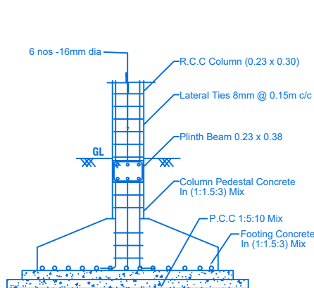
COLUMN FOOTING DETAILS
