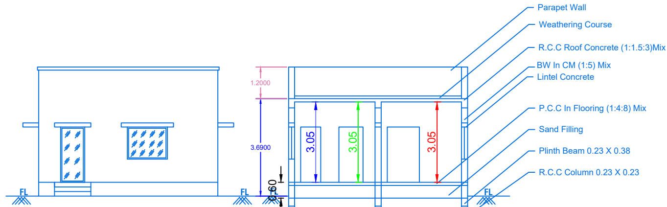
FRONT ELEVATION
