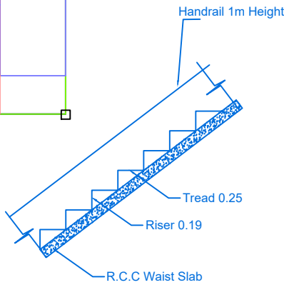
STAIR DETAILS
