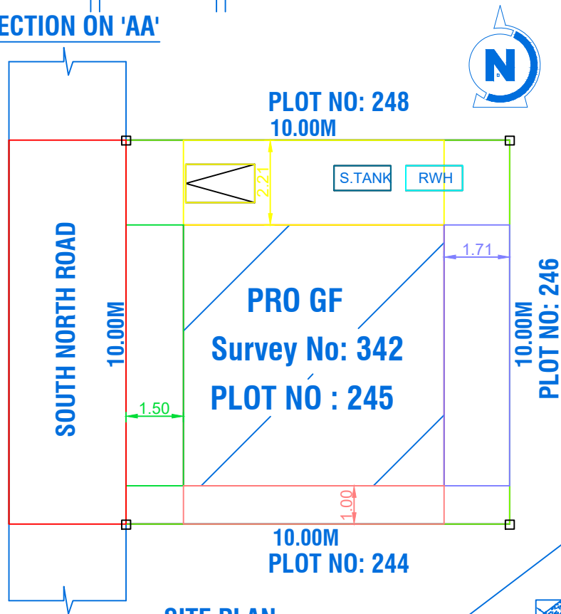
SITE PLAN
