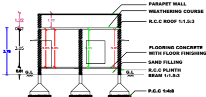
SECTION ON AA SECTION ON AA
