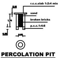
PERCOLATION PIT
