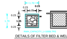
DETAILS OF FILTER BED & WELL
