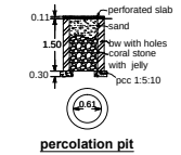
percolation pit
