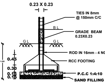
RCC COLUMN DETAILS
