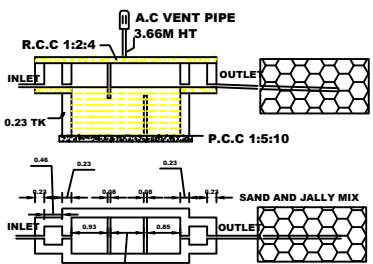
SEPTIC TANK AND TRENCH
