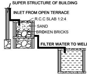
RAINWATER HARVESTING
