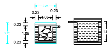
DETAILS OF FILTER BED & WELL
