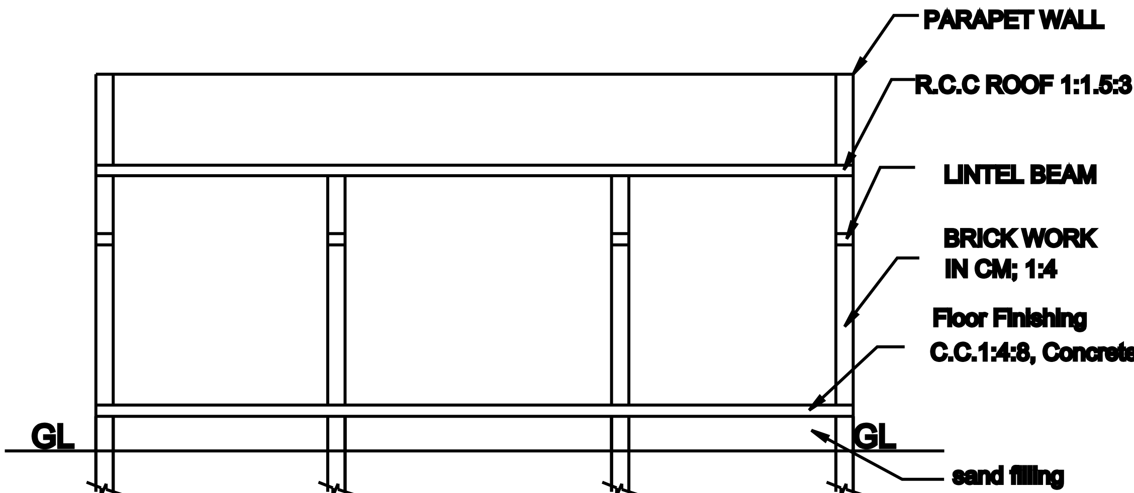
SECTION NN
