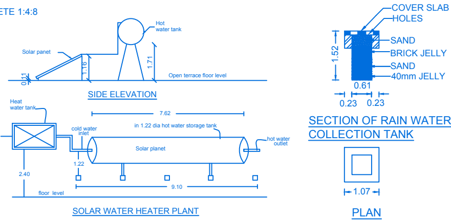
SOLAR WATER HEATER PLANT
