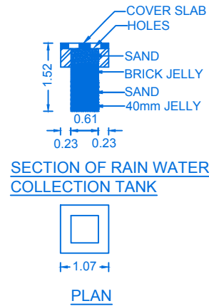
PLAN
