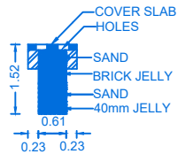
SECTION OF RAIN WATER COLLECTION TANK
