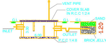
SECTION-AB
