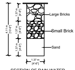
SECTION OF RAIN WATER COLLECTION PITS (NTS)
