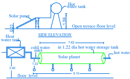
SOLAR WATER HEATER PLANT
