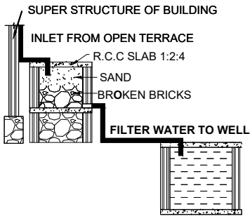
RAINWATER HARVESTING
