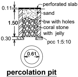
percolation pit
