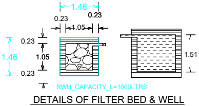
RAINWATER HARVESTING
