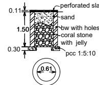
percolation pit
