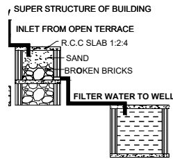
RAINWATER HARVESTING
