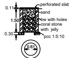
percolation pit
