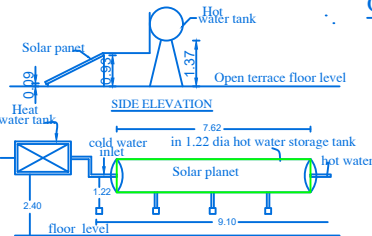
SOLAR WATER HEATER PLANT
