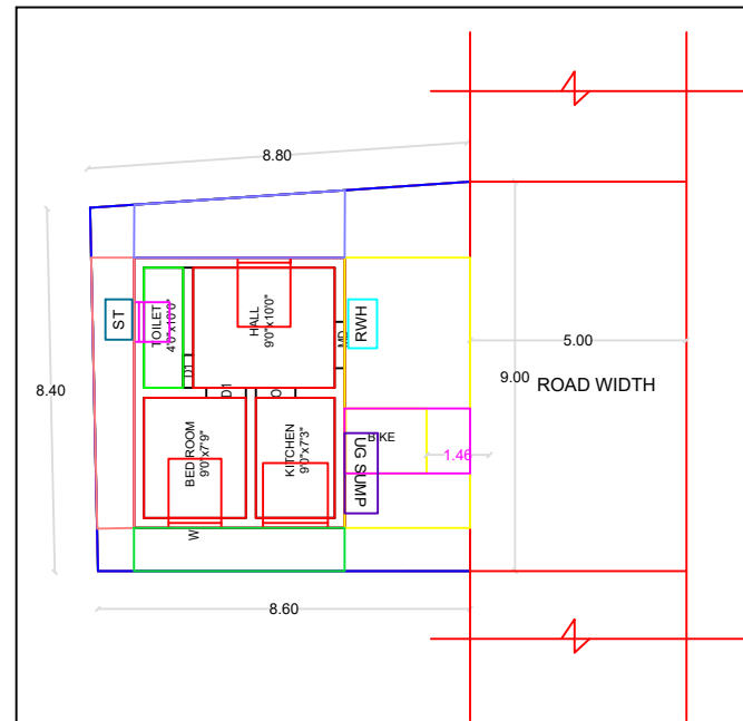
RESIDUARY PLOT SKETCH, SUPER IMPOSED (SITE PLAN)
