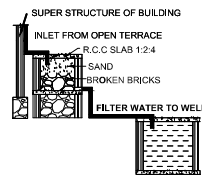
RAINWATER HARVESTING
