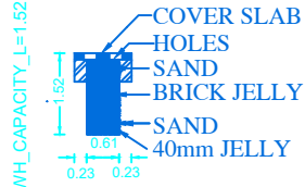
SECTION OF RAIN WATER COLLECTION TANK
