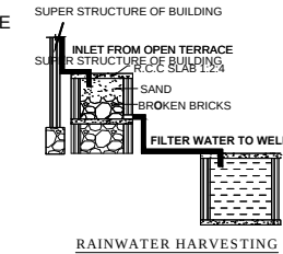
RAINWATER HARVESTING
