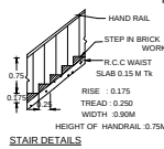
STAIR DETAILS
