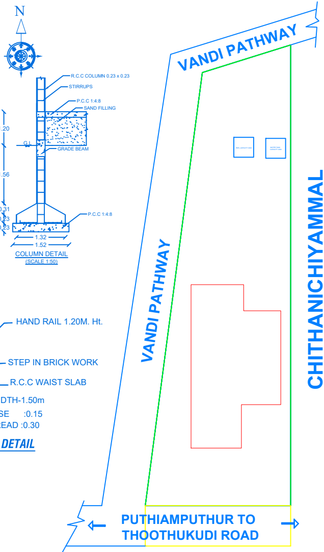
SITE PLAN
