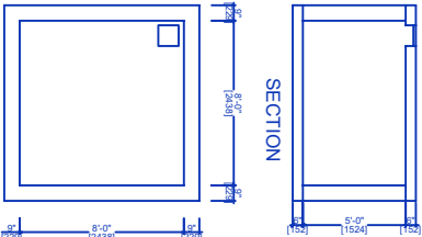
DETAILS OF COLLECTION SUMP FOR RAIN
