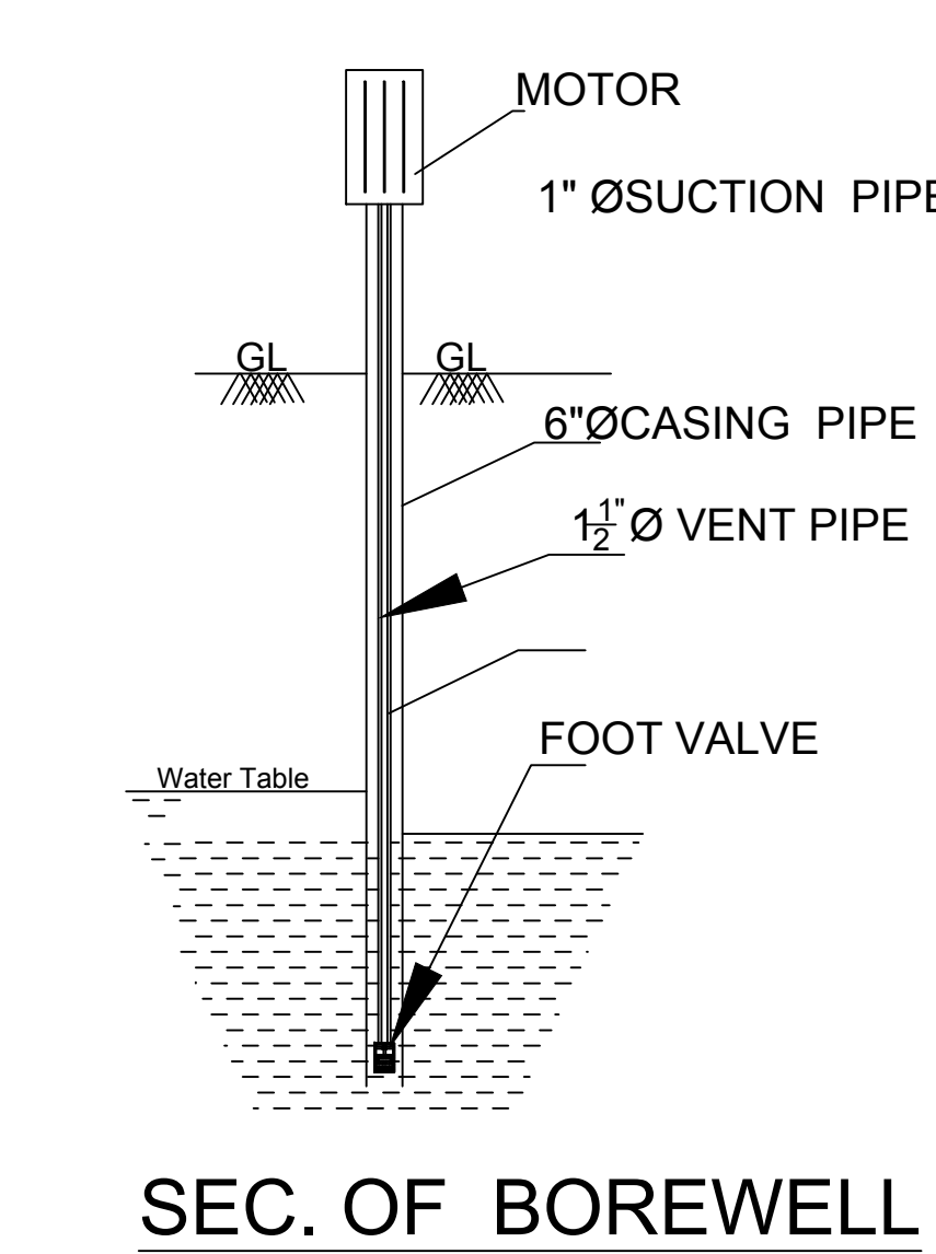
SEC. OF BOREWELL
