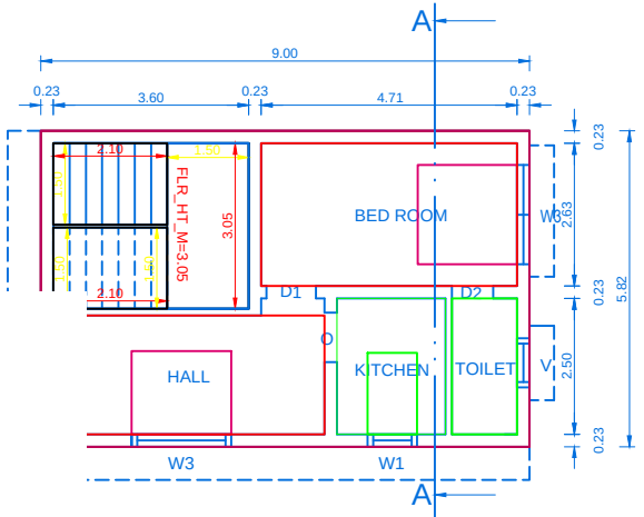
PROP.FIRST FLOOR PLAN
