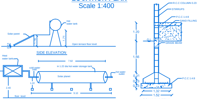
SOLAR WATER HEATER PLANT
