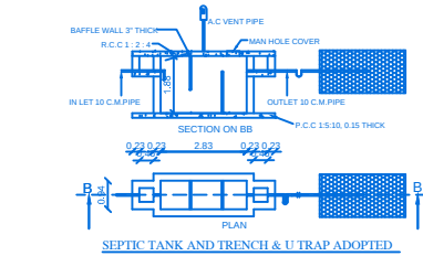
SEPTIC TANK AND TRENCH & U TRAP ADOPTED
