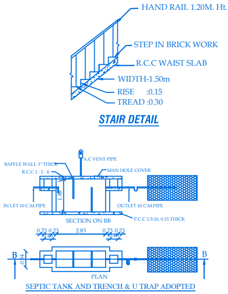
SEPTIC TANK AND TRENCH & U TRAP ADOPTED
