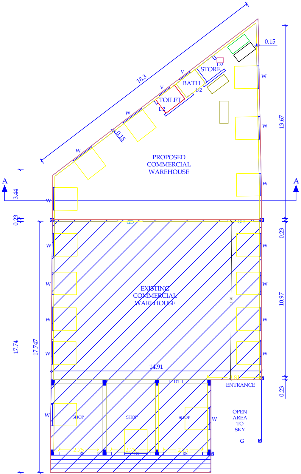
EXG & PRO GROUND FLOOR PLAN
