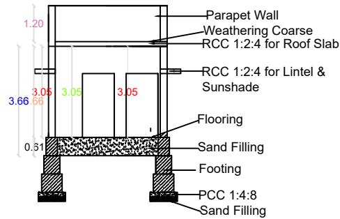
SECTION AB
