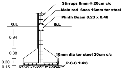
Details of column footing
