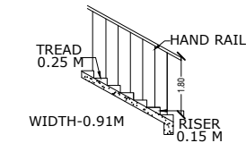
STAIRCASE DETAILS
