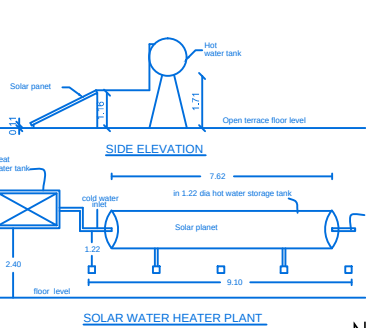
SOLAR WATER HEATER PLANT
