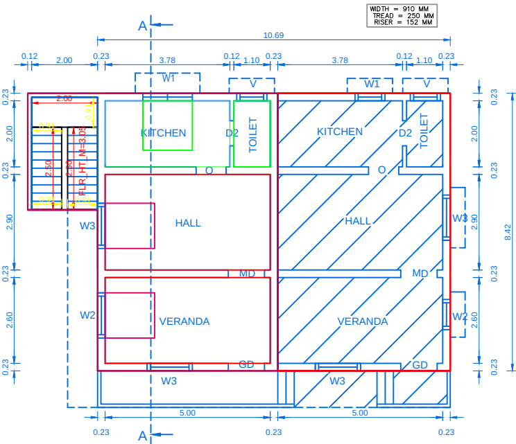
EXG & PROP.GROUND FLOOR PLAN
