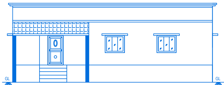
FRONT ELEVATION
