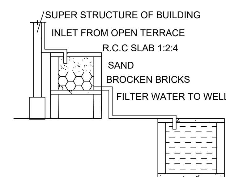
RAINWATER HARVESTING
