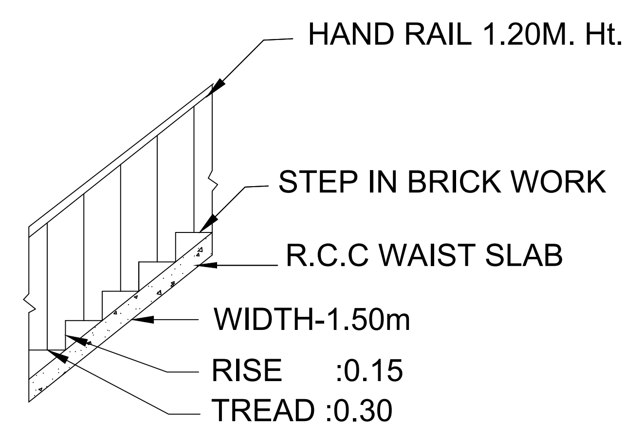
STAIR DETAIL
