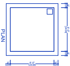
DETAILS OF COLLECTION SUMP FOR RAIN WATER HARVESTING OF ROOF TOP RAIN WATER RWH_CAPACITY_L=5000LTRS
