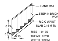
STAIR DETAILS
