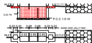
SEPTIC TANK AND TRENCH
