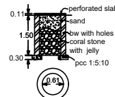
percolation pit
