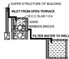
RAINWATER HARVESTING
