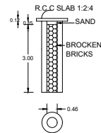
PERCOLATION PIT
