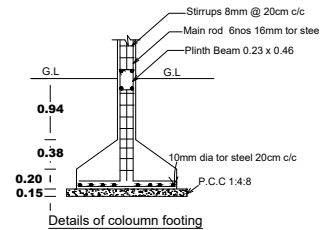
Details of column footing
