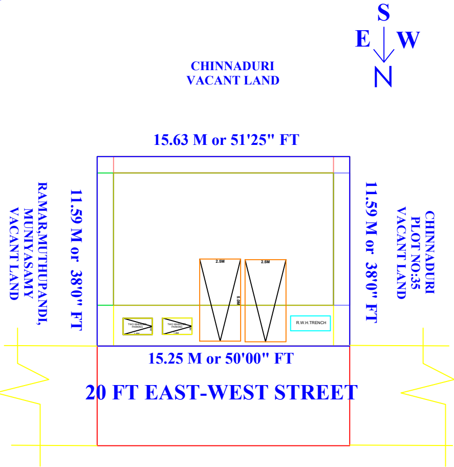
SITE PLAN
