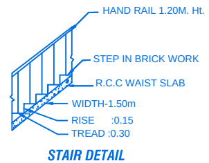
STAIR DETAIL
