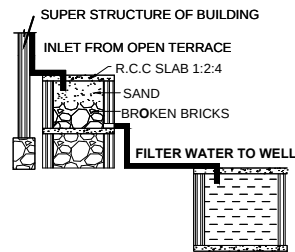
RAINWATER HARVESTING
