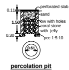
percolation pit
