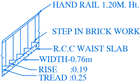
STAIR DETAIL
