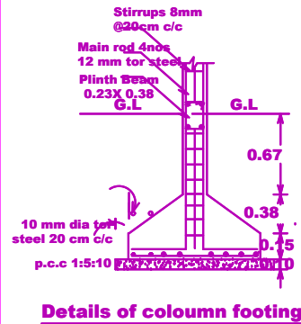
Details of column footing
