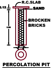
PERCOLATION PIT
