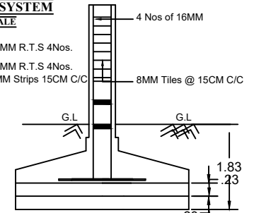
RCC COLUMN DETAILS
