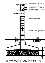
RCC COLUMN DETAILS
